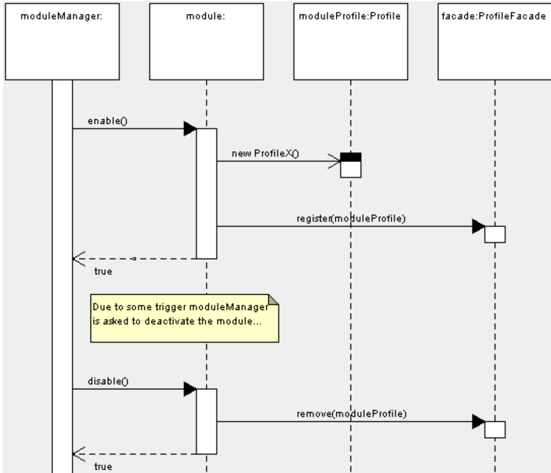
Figure 5.8. Sequence diagram of the registering and unregistering of a profile
