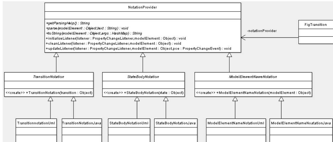
Figure 5.3. Notation subsystem part 2.
