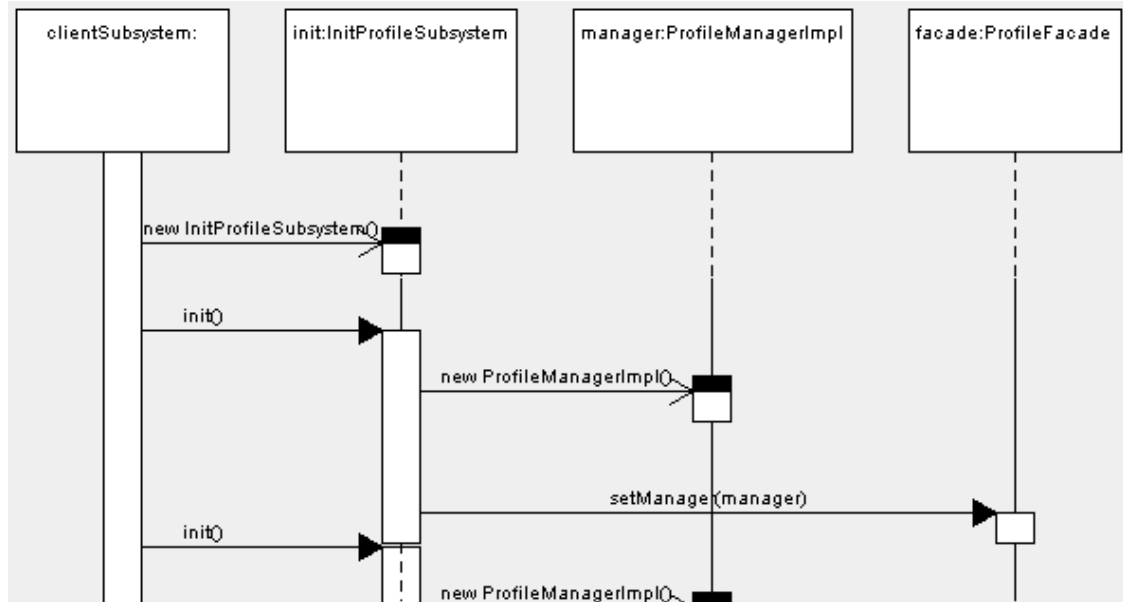
Figure 5.6. Sequence diagram of the profile subsystem initialization.
