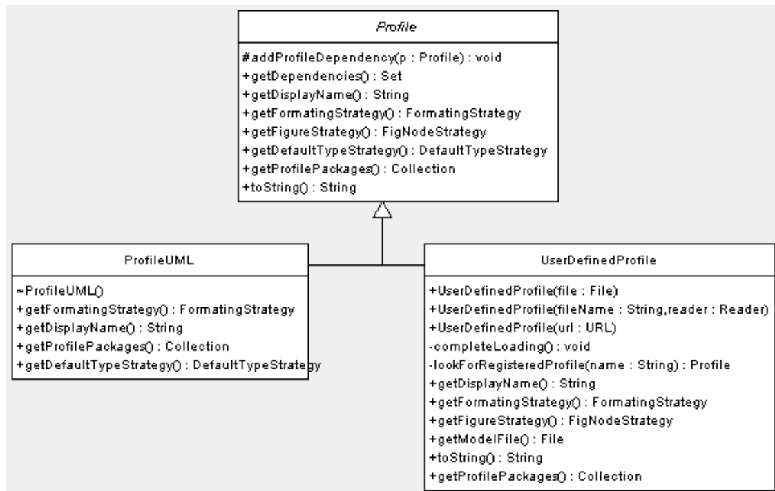
Figure 5.7. Class diagram of the Profile class and some derived classes
