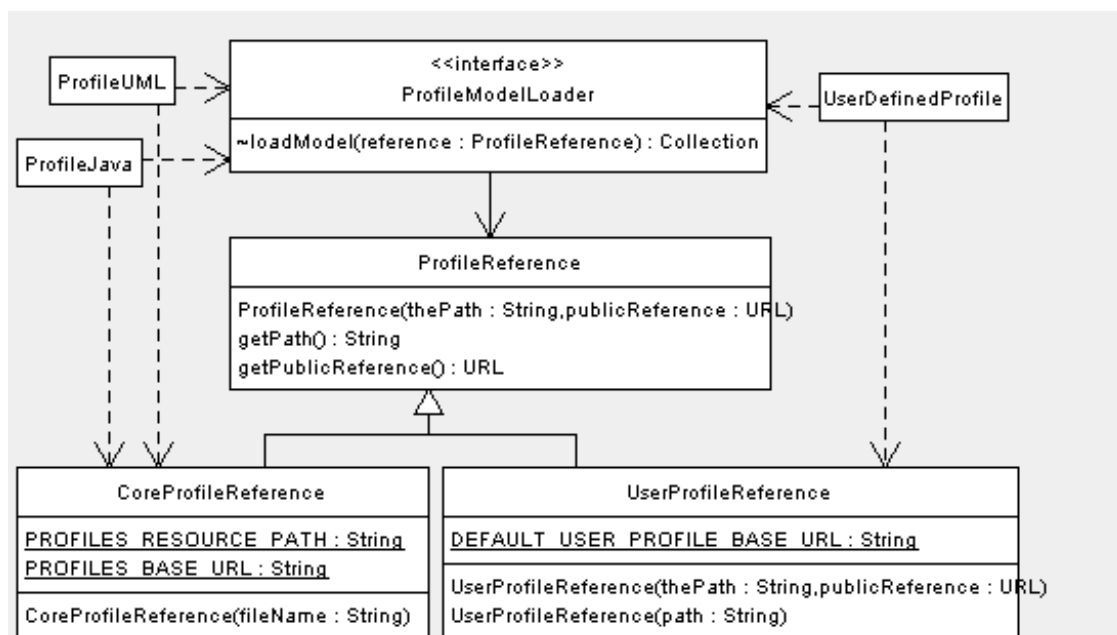
Figure 5.9. Class diagram of the ProfileReference class and associated classes
